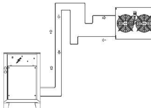
Dehumidifier lower than the condenser
