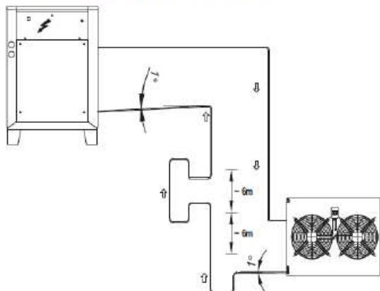
Dehumidifier higher than the condenser
